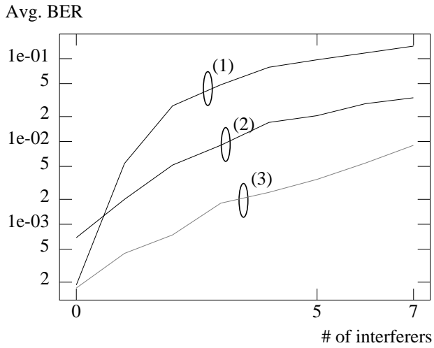
Fig. 6 Average BER vs. # of interferers for spreading factor N = 8 with Rayleigh fading and SNR=10dB . Simulation results for (1) Maximal Ratio Combining (2) Equal Gain Combining (3) Wiener filtering.
