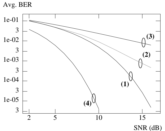
Fig. 3 Average BER vs. SNR with Rayleigh fading and a full load for Wiener Filtering: (1) analytical, N \rightarrow \text{INF} , (2) simulation, N = 8 , (3) analytical, N = 1 (single narrowband), and (4) analytical, N = 1 with linear time invariant AWGN channel.
