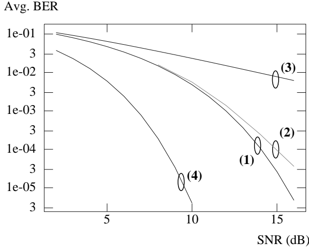
Fig. 4 Average BER vs. SNR with Rayleigh fading and a full load for Wiener Filtering: (1) analytical, N \rightarrow \infty , (2) simulation, N = 64 , (3) analytical, N = 1 (single narrowband), and (4) analytical, N = 1 with linear time invariant AWGN channel.
