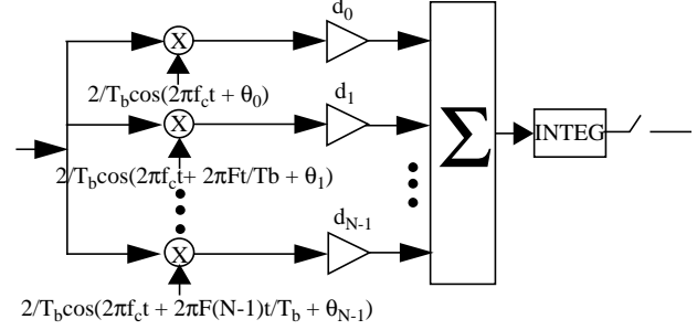
Fig. 2 Receiver Model
