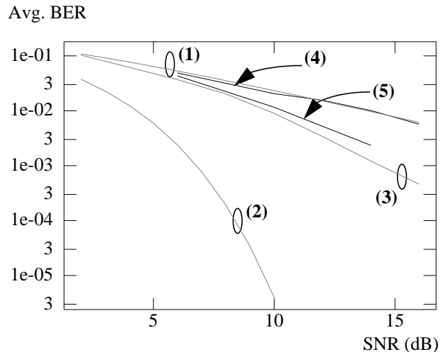
Fig. 5 Average BER vs. SNR with Rayleigh fading and a full load for Wiener filtering: (1) analytical, N = 1 (single subcarrier), (2) analytical, N = 1 with linear time invariant AWGN channel, (3) simulation, N = 8 with iid fading ( \alpha = \infty ), (4) simulation, N = 8 , correlated fading with \alpha = 0.001 ( L = 1 ) and (5) \alpha = 0.125 ( L = 2 ).
