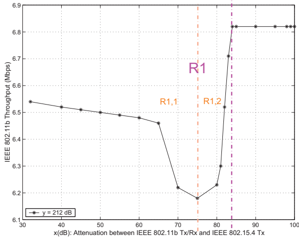
Fig. 6. In R1: IEEE 802.11b/g nodes can also sense IEEE 802.15.4 traffic
