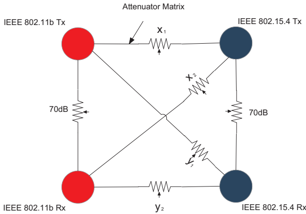
Fig. 5. Functional diagram of the coexistence testbed
