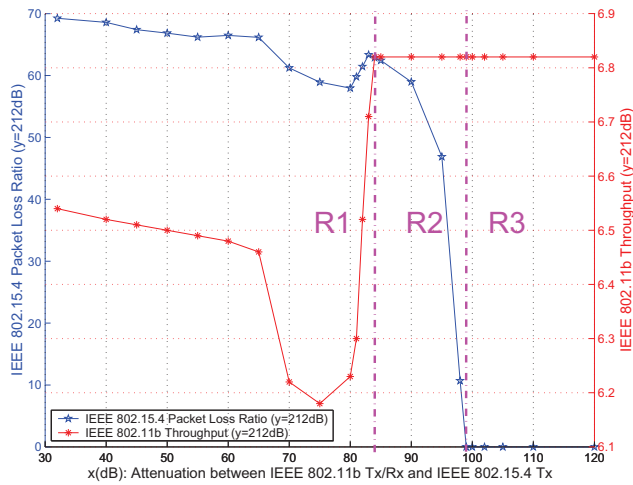
Fig. 9. In R2: IEEE 802.15.4 nodes can sense IEEE 802.11b/g nodes, but not vice versa
