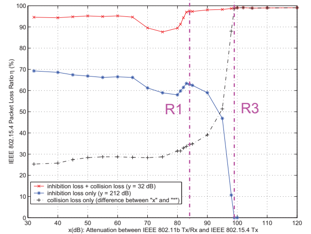
Fig. 8. In R3: neither can sense the other, but IEEE 802.15.4 nodes could still suffer IEEE 802.11b/g interference
