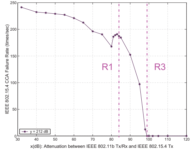
Fig. 7. IEEE 802.15.4 Tx CCA Failure Rate
