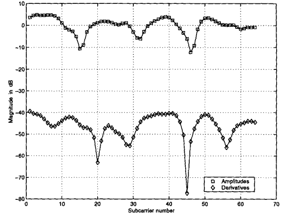
Figure 2: Amplitudes |V + \zeta_0 V' T| and derivatives |V' T| , as a function of subcarrier number for a sample channel
