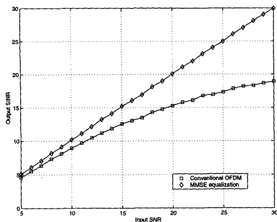
Figure 4: SINR before the slicer, versus input SINR for conventional OFDM receiver and our newly proposed system.
